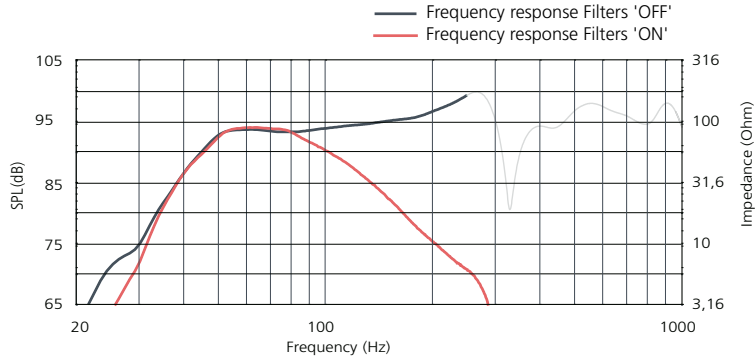
Frequency response 'on axis'
