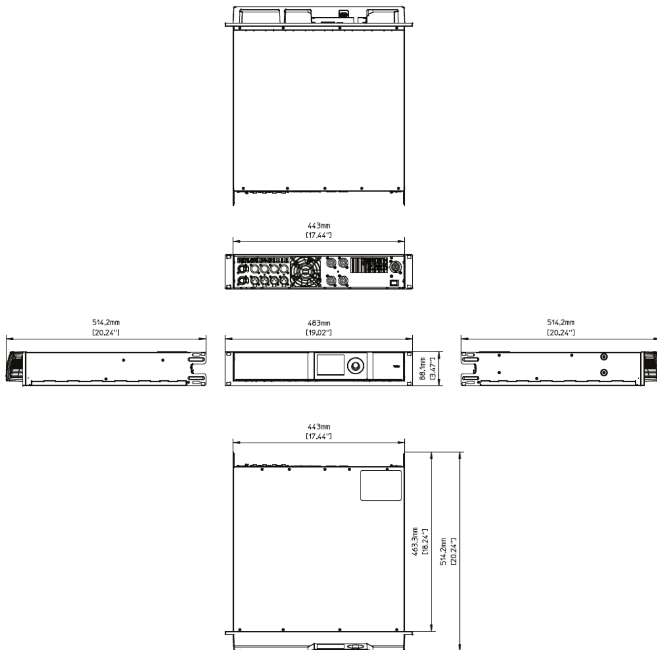
Figure 8.2: Dimensions: TGX
